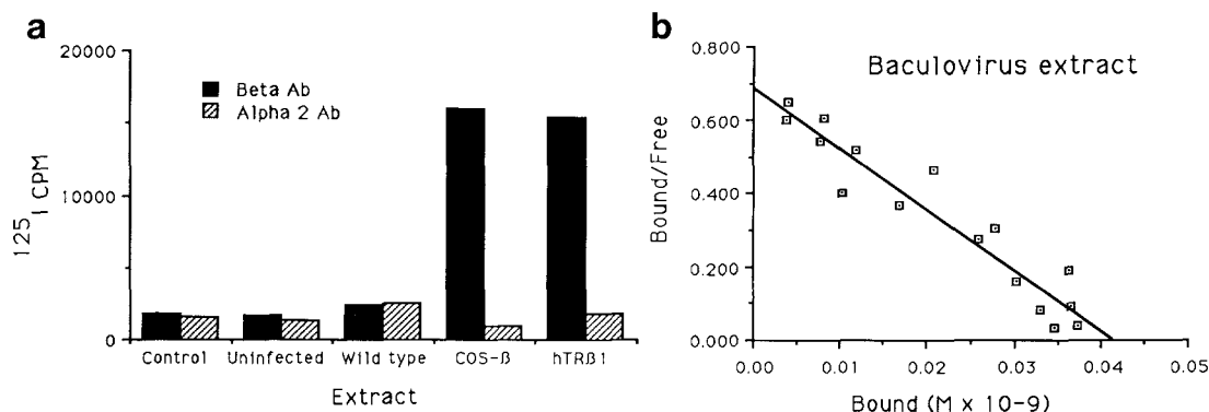
Fig. 2a. [ 125 I]-T3 binding profiles of immunoprecipitated human thyroid hormone receptor β1 produced in Baculovirus-infected insect cells or in COS cells. Extracts from independent isolates of recombinant baculovirus-infected cells were examined for expression of hTRβ1 using immunoprecipitation with either a specific anti-hTRβ1 antibody or with an antibody specific for the hTRα2 splicing variant. In this figure, only one of the extracts containing the 55 kDa protein is shown. For comparison, an extract of hTRβ1 expressed in COS cells was used as a positive control. The various extracts (7.5 μl) were incubated with 0.5 nM [ 125 I]-T3 and immunoprecipitated with anti-hTRβ1 or anti-hTRα2 anti-peptide antibody and protein A/G agarose beads.
